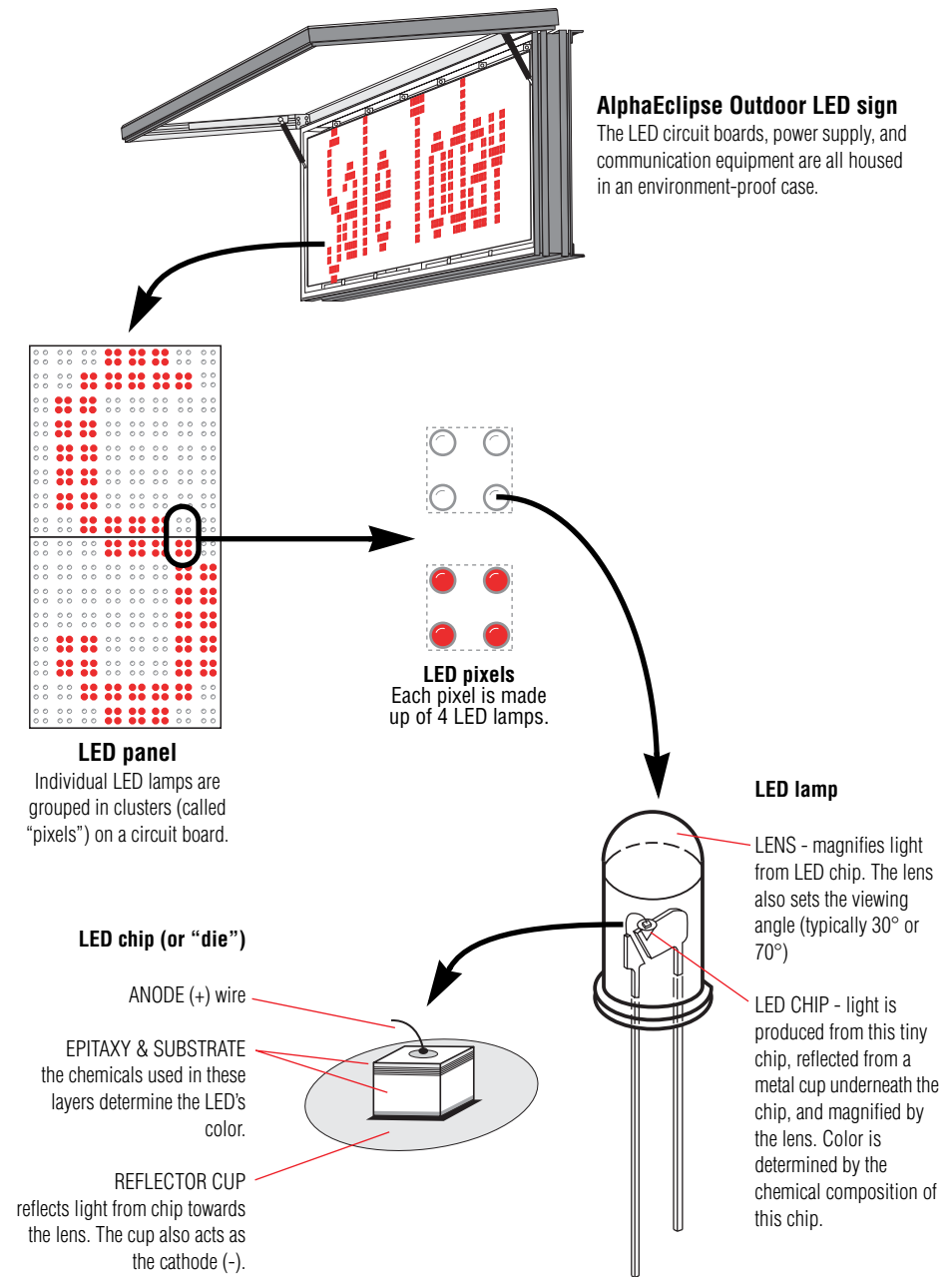
FIGURE 7. AlphaEclipse™ outdoor LED sign
